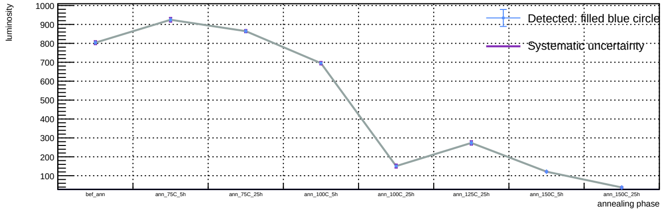
Sensor A1, v = 5 V, representative T = 23 C (max available) - Spot 0: luminosity vs phase
