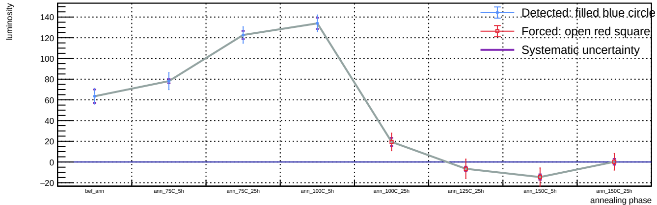
Sensor A1, v = 5 V, representative T = 23 C (max available) - Spot 2: luminosity vs phase
