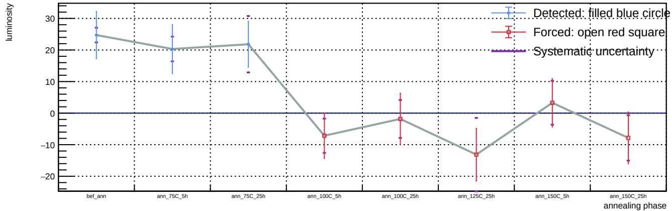
Sensor A1, v = 5 V, representative T = 23 C (max available) - Spot 21: luminosity vs phase
