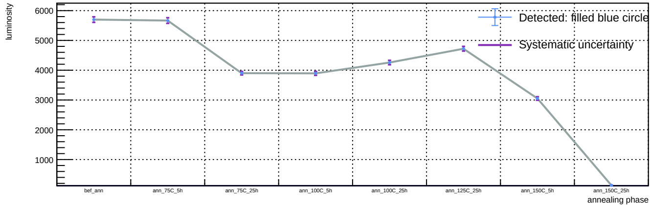
Sensor A1, v = 5 V, representative T = 23 C (max available) - Spot 3: luminosity vs phase
