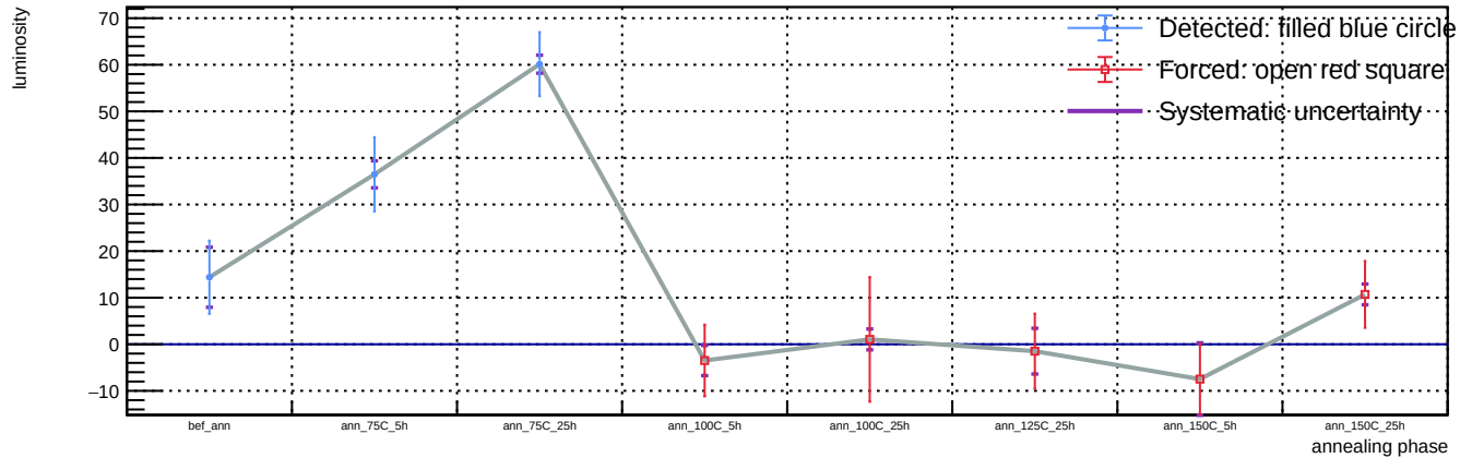
Sensor A1, v = 5 V, representative T = 23 C (max available) - Spot 44: luminosity vs phase
