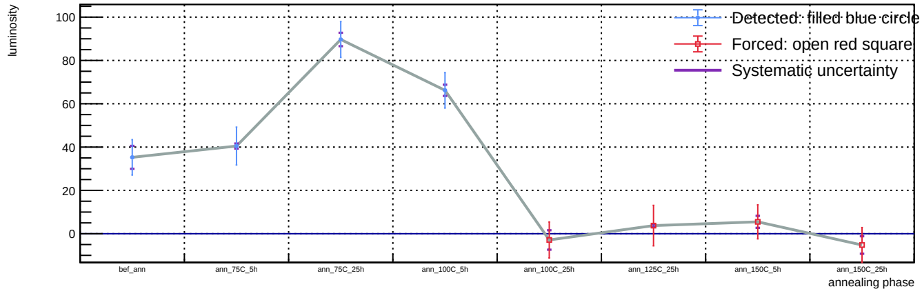
Sensor A1, v = 5 V, representative T = 23 C (max available) - Spot 47: luminosity vs phase
