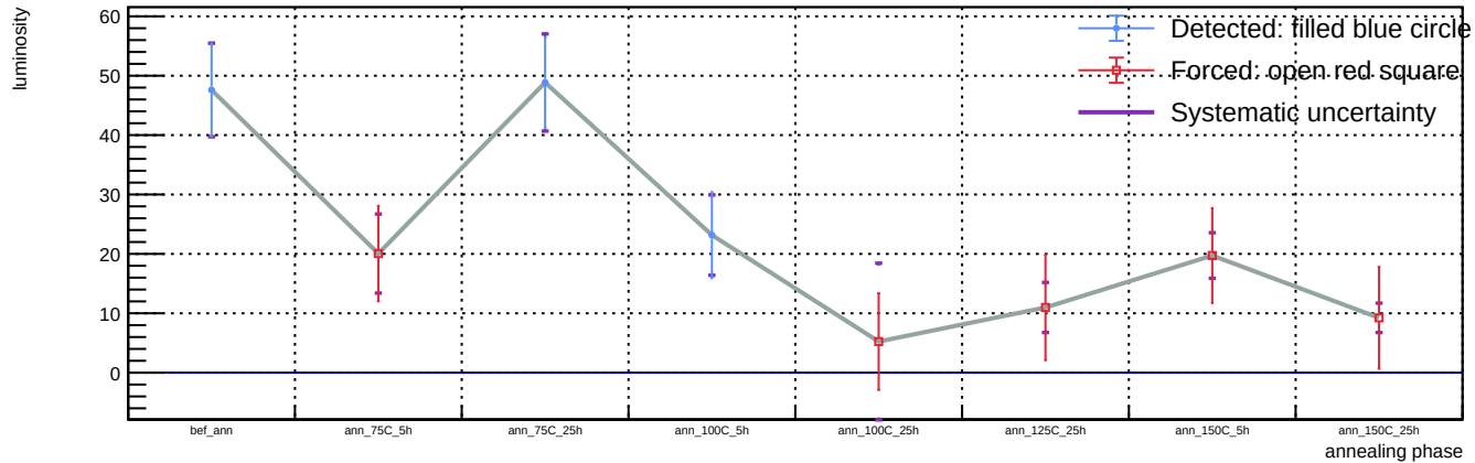
Sensor A1, v = 5 V, representative T = 23 C (max available) - Spot 5: luminosity vs phase
