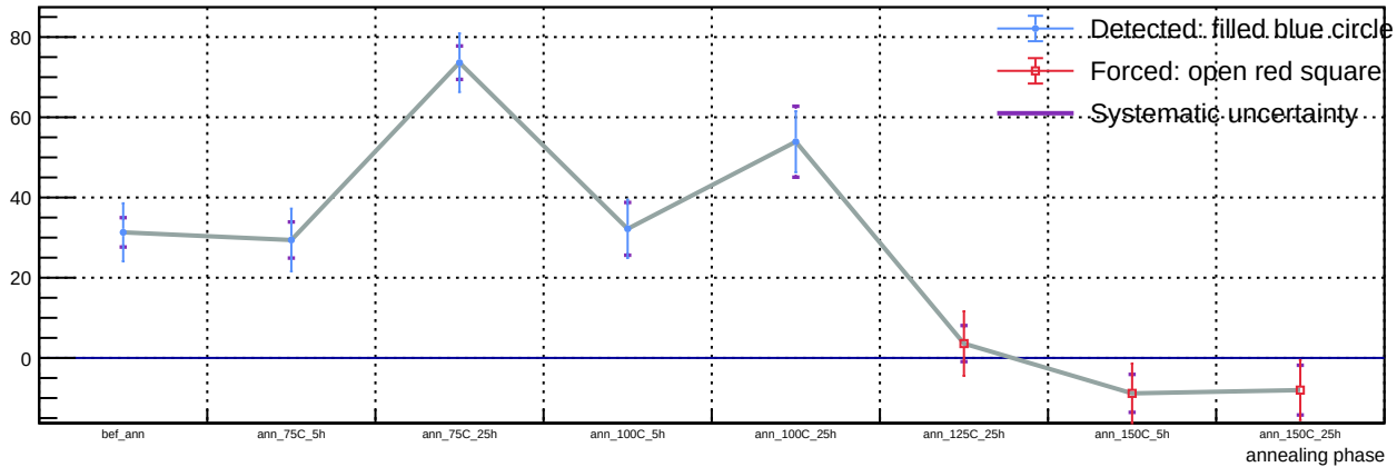
Sensor A1, v = 5 V, representative T = 23 C (max available) - Spot 53: luminosity vs phase
