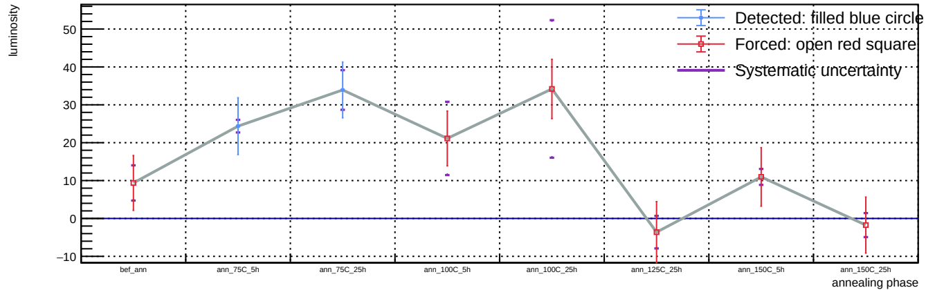
Sensor A1, v = 5 V, representative T = 23 C (max available) - Spot 63: luminosity vs phase
