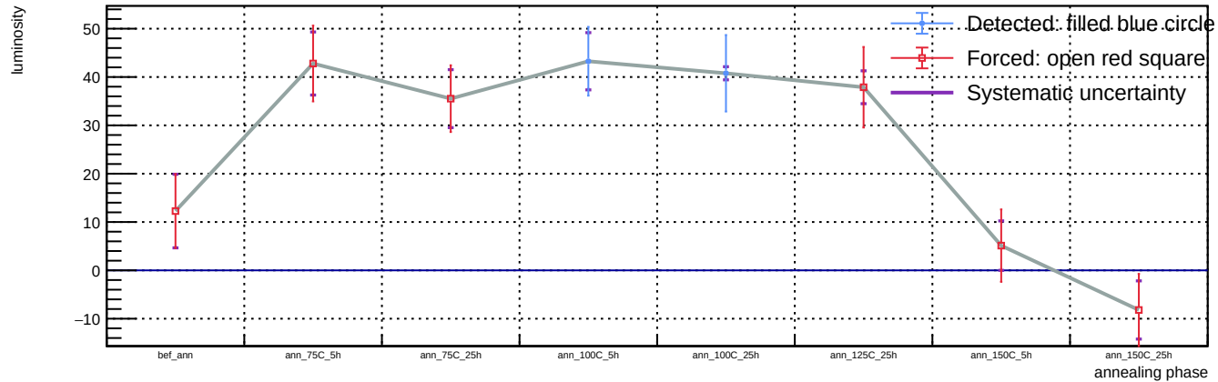
Sensor A1, v = 5 V, representative T = 23 C (max available) - Spot 66: luminosity vs phase
