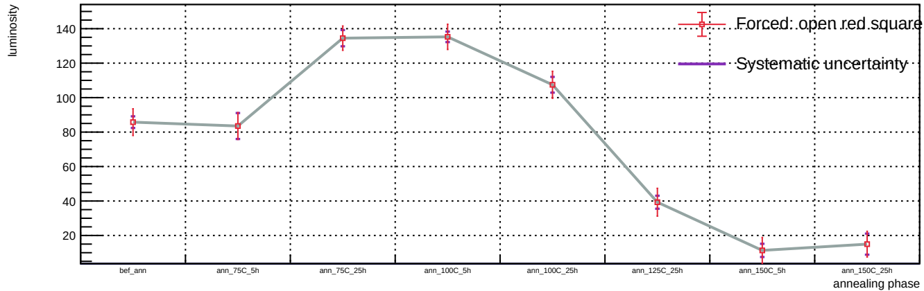
Sensor A1, v = 5 V, representative T = 23 C (max available) - Spot 82: luminosity vs phase
