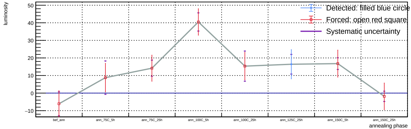
Sensor A1, v = 5 V, representative T = 23 C (max available) - Spot 84: luminosity vs phase
