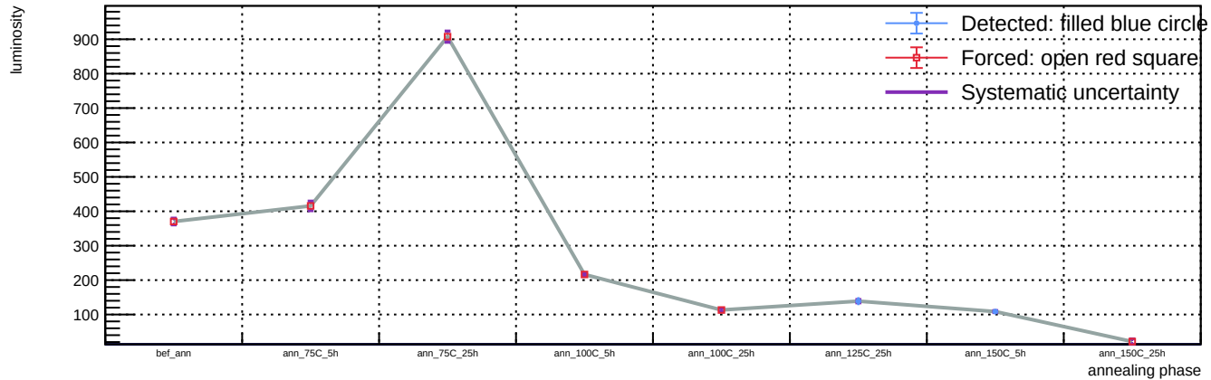
Sensor A1, v = 5 V, representative T = 23 C (max available) - Spot 87: luminosity vs phase
