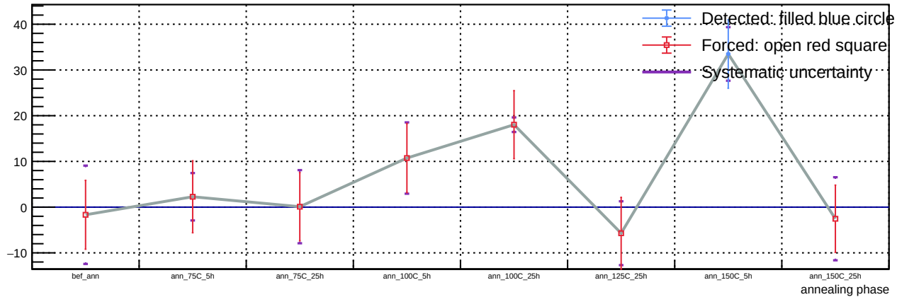
Sensor A1, v = 5 V, representative T = 23 C (max available) - Spot 90: luminosity vs phase
