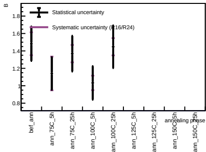
Sensor B1, T = 20 C - Spot 3
