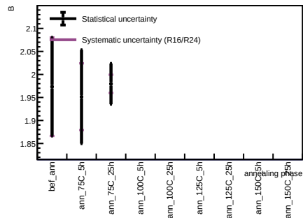
Sensor B1, T = 20 C - Spot 2
