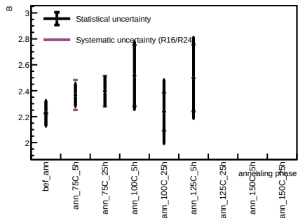
Sensor B1, T = 20 C - Spot 1
