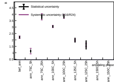
Sensor B1, T = 20 C - Spot 5
