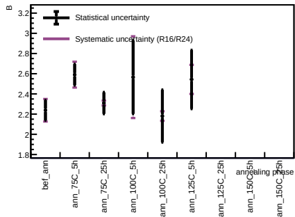
Sensor B1, T = 20 C - Spot 4
