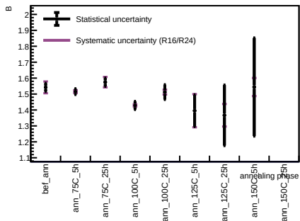
Sensor B1, T = 20 C - Spot 0
