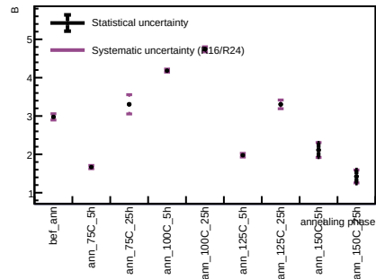
Sensor B1, T = 20 C - Spot 11
