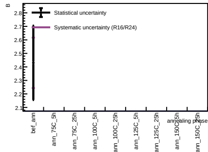
Sensor B1, T = 20 C - Spot 8
