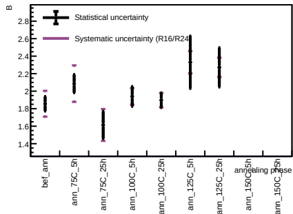
Sensor B1, T = 20 C - Spot 10
