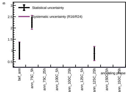
Sensor B1, T = 20 C - Spot 7
