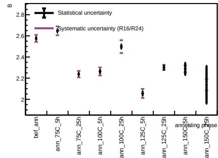
Sensor B1, T = 20 C - Spot 34
