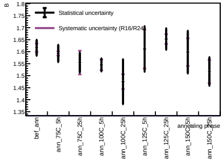
Sensor B1, T = 20 C - Spot 31
