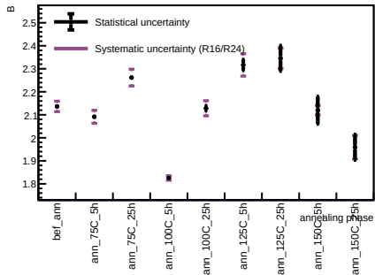
Sensor B1, T = 20 C - Spot 30
