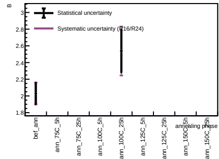
Sensor B1, T = 20 C - Spot 35
