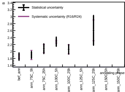
Sensor B1, T = 20 C - Spot 33
