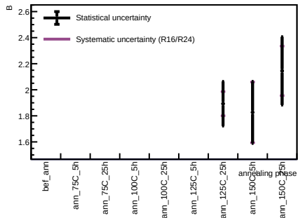
Sensor B1, T = 20 C - Spot 106
