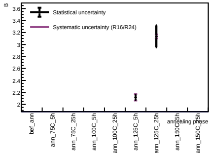
Sensor B1, T = 20 C - Spot 102
