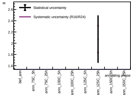
Sensor B1, T = 20 C - Spot 103
