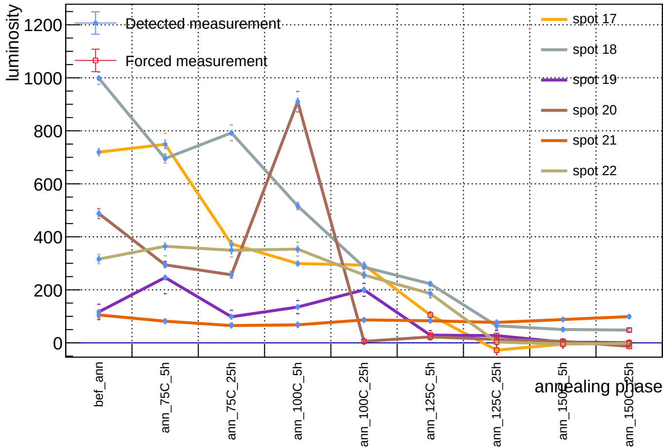
Sensor B1, T = 20 C, representative v = 55.9 V (max available) - luminosity vs phase - order 10^2
