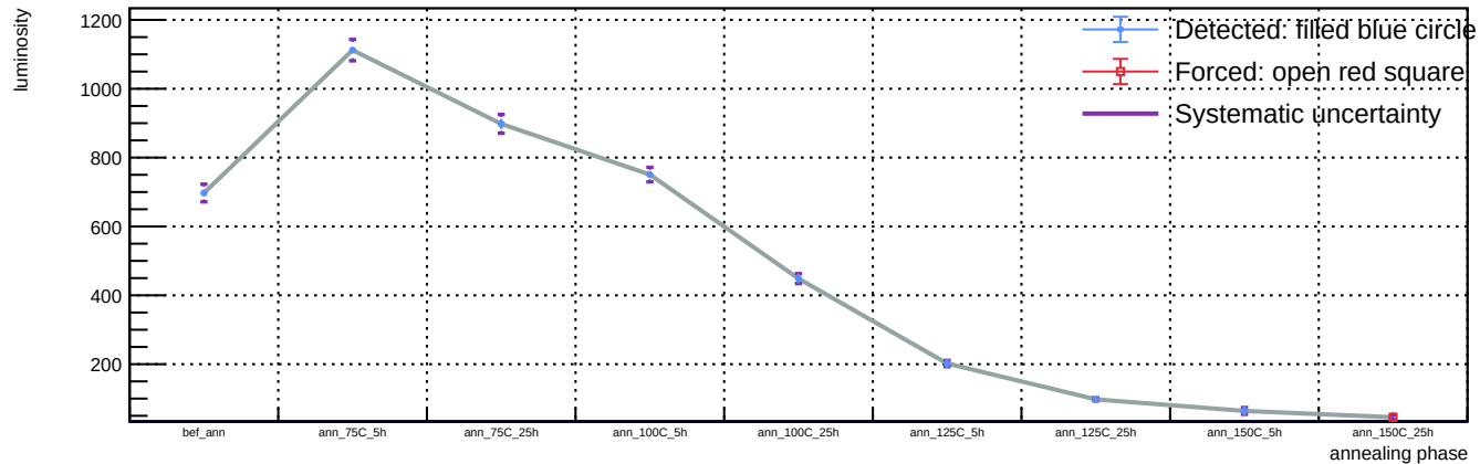
Sensor B1, T = 20 C, representative v = 55.9 V (max available) - Spot 0: luminosity vs phase
