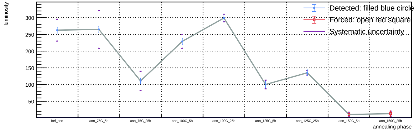
Sensor B1, T = 20 C, representative v = 55.9 V (max available) - Spot 10: luminosity vs phase
