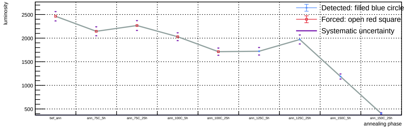
Sensor B1, T = 20 C, representative v = 55.9 V (max available) - Spot 101: luminosity vs phase
