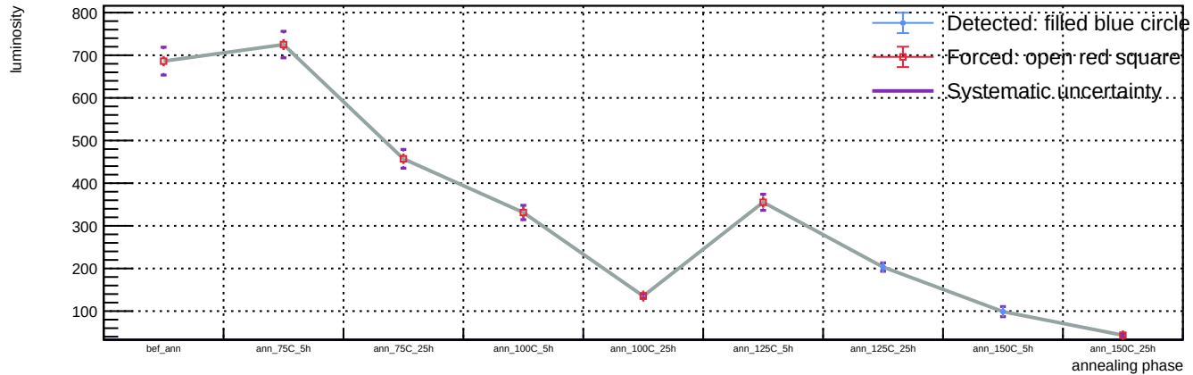
Sensor B1, T = 20 C, representative v = 55.9 V (max available) - Spot 105: luminosity vs phase
