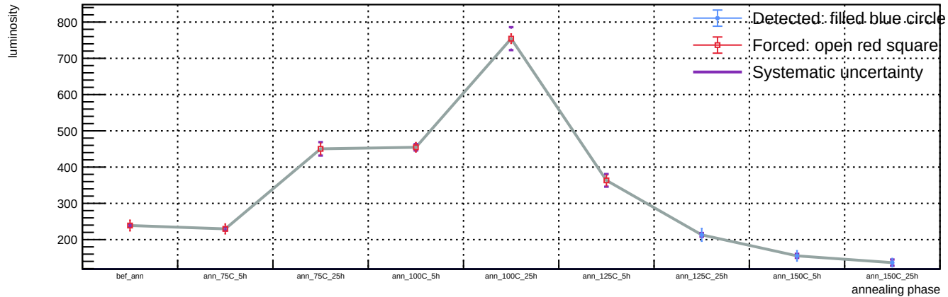
Sensor B1, T = 20 C, representative v = 55.9 V (max available) - Spot 106: luminosity vs phase
