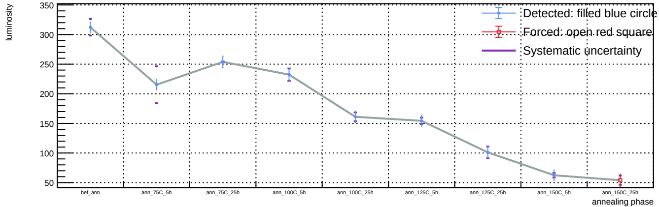
Sensor B1, T = 20 C, representative v = 55.9 V (max available) - Spot 12: luminosity vs phase
