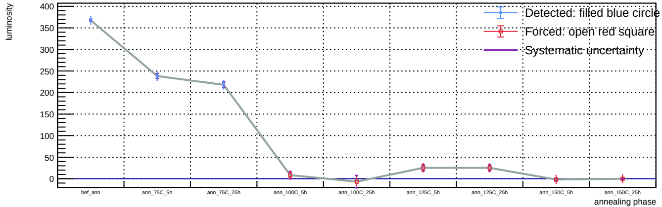
Sensor B1, T = 20 C, representative v = 55.9 V (max available) - Spot 13: luminosity vs phase
