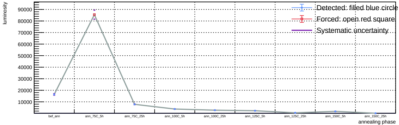
Sensor B1, T = 20 C, representative v = 55.9 V (max available) - Spot 14: luminosity vs phase
