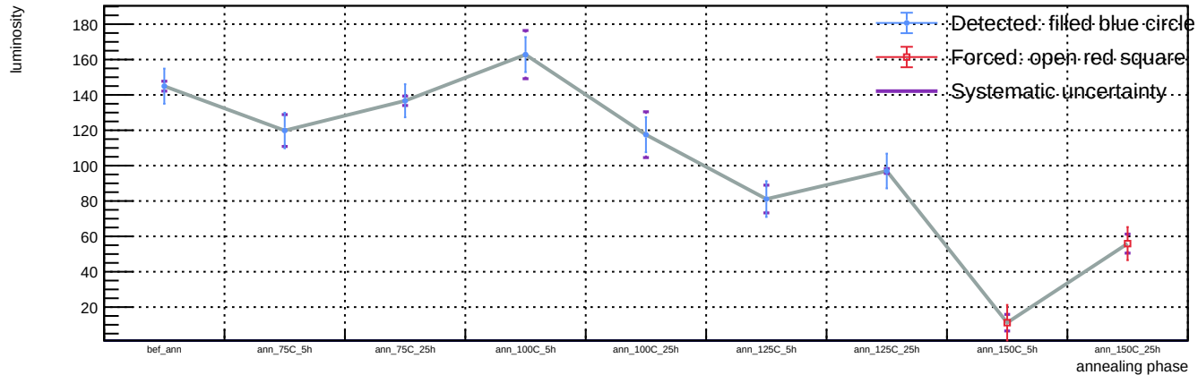
Sensor B1, T = 20 C, representative v = 55.9 V (max available) - Spot 15: luminosity vs phase
