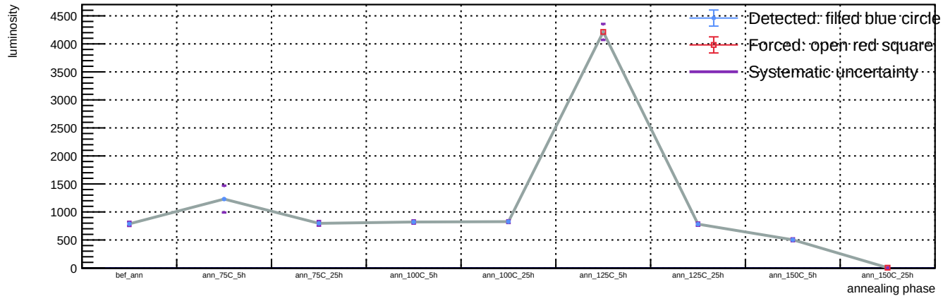
Sensor B1, T = 20 C, representative v = 55.9 V (max available) - Spot 16: luminosity vs phase
