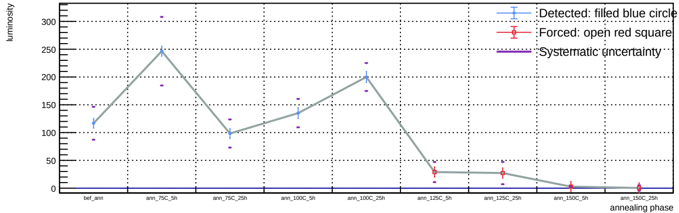
Sensor B1, T = 20 C, representative v = 55.9 V (max available) - Spot 19: luminosity vs phase
