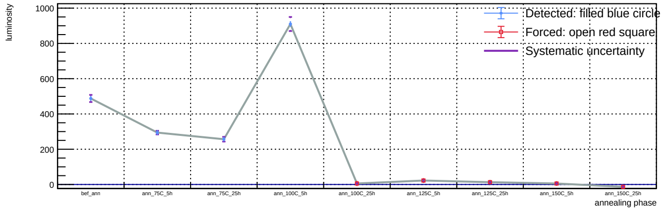
Sensor B1, T = 20 C, representative v = 55.9 V (max available) - Spot 20: luminosity vs phase
