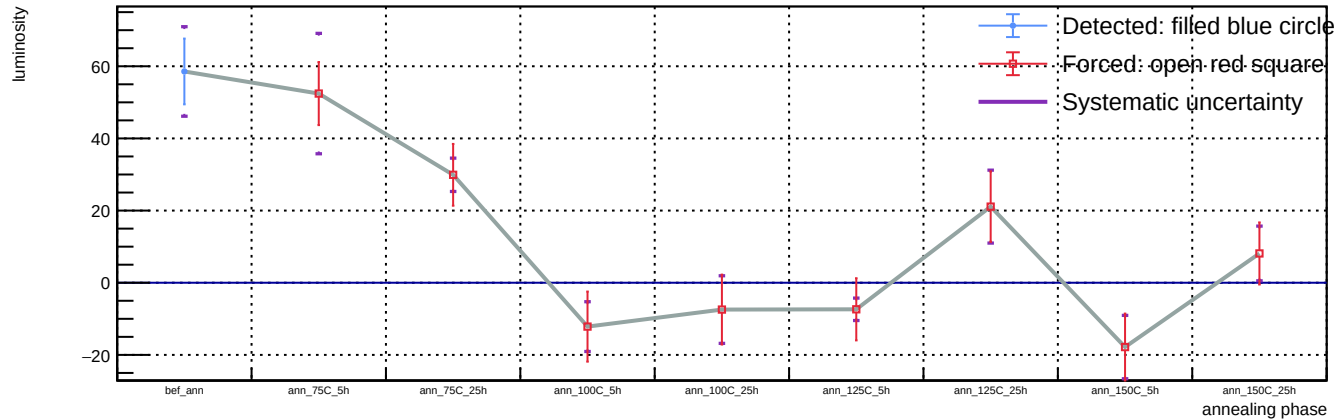
Sensor B1, T = 20 C, representative v = 55.9 V (max available) - Spot 24: luminosity vs phase
