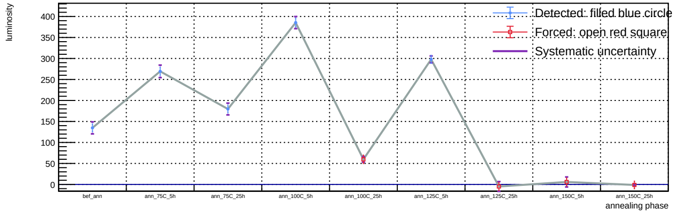
Sensor B1, T = 20 C, representative v = 55.9 V (max available) - Spot 28: luminosity vs phase
