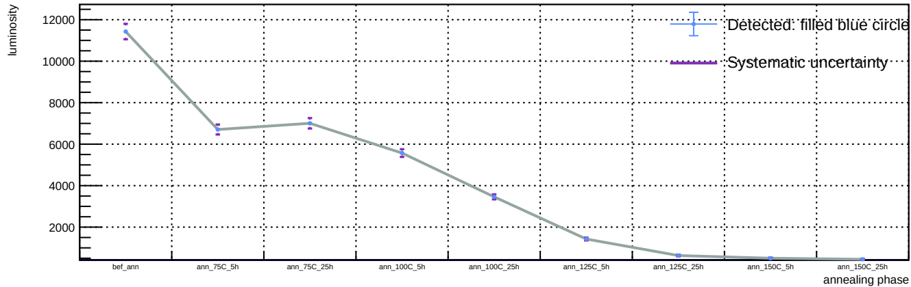
Sensor B1, T = 20 C, representative v = 55.9 V (max available) - Spot 30: luminosity vs phase
