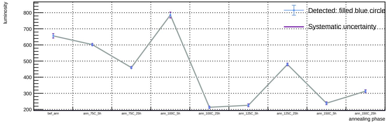
Sensor B1, T = 20 C, representative v = 55.9 V (max available) - Spot 31: luminosity vs phase
