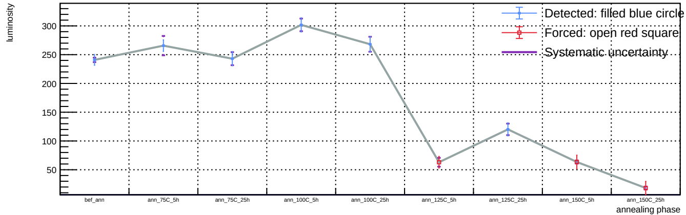
Sensor B1, T = 20 C, representative v = 55.9 V (max available) - Spot 33: luminosity vs phase
