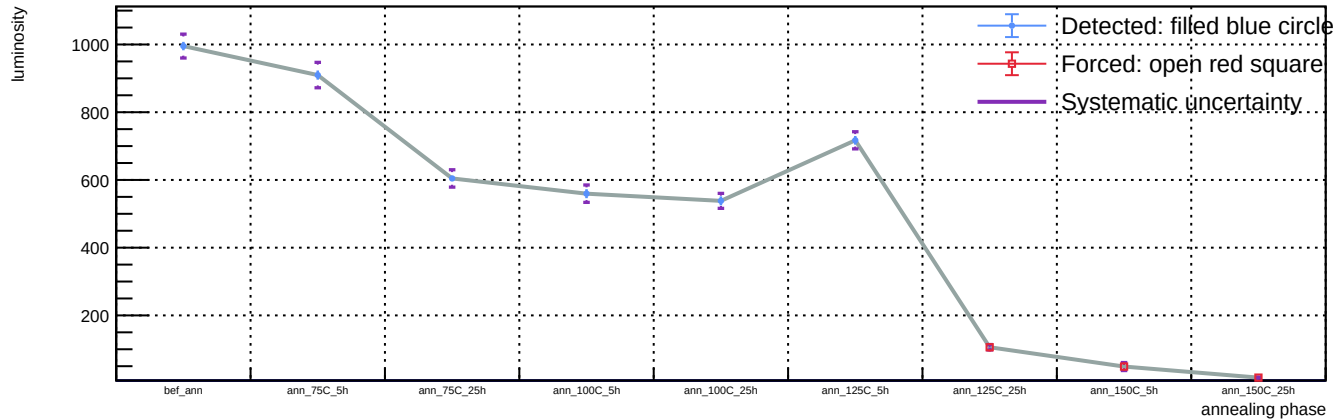
Sensor B1, T = 20 C, representative v = 55.9 V (max available) - Spot 38: luminosity vs phase
