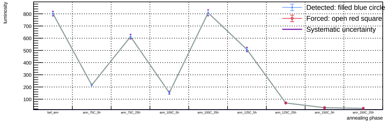
Sensor B1, T = 20 C, representative v = 55.9 V (max available) - Spot 40: luminosity vs phase
