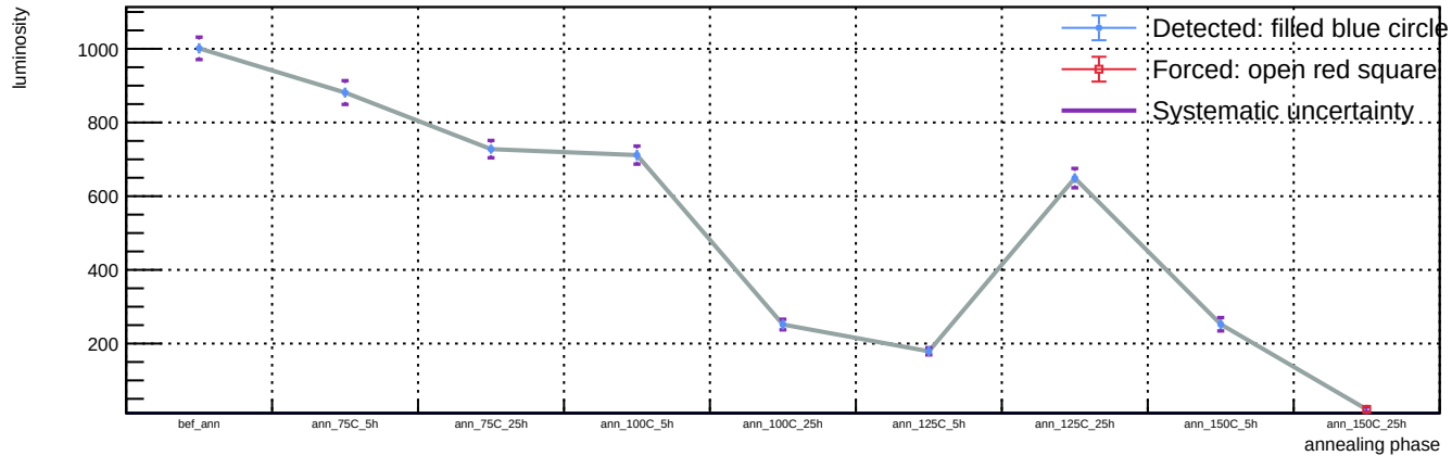
Sensor B1, T = 20 C, representative v = 55.9 V (max available) - Spot 45: luminosity vs phase
