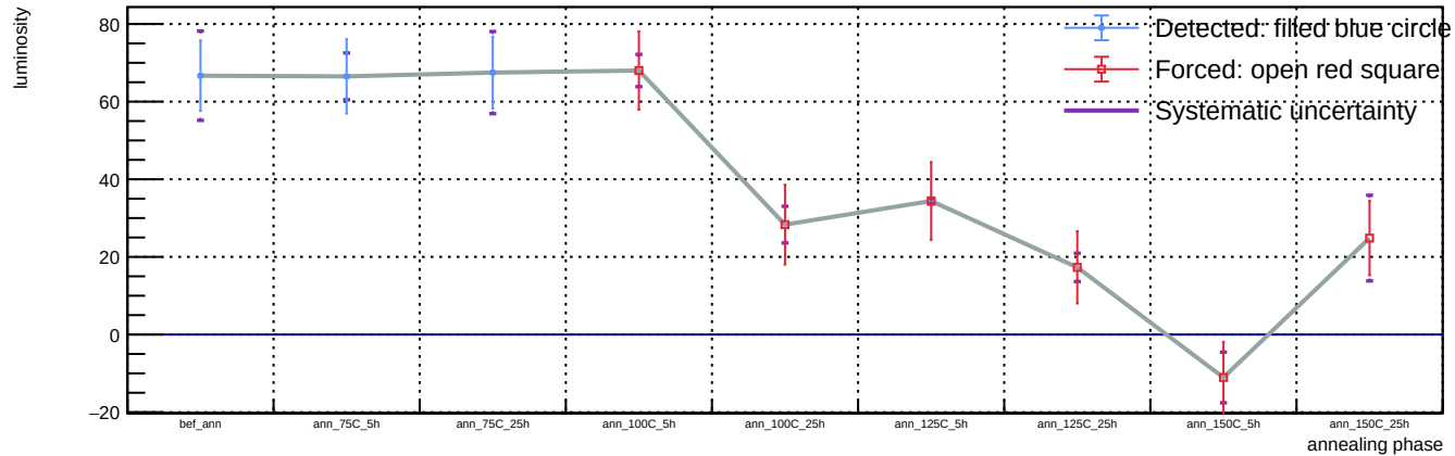
Sensor B1, T = 20 C, representative v = 55.9 V (max available) - Spot 50: luminosity vs phase
