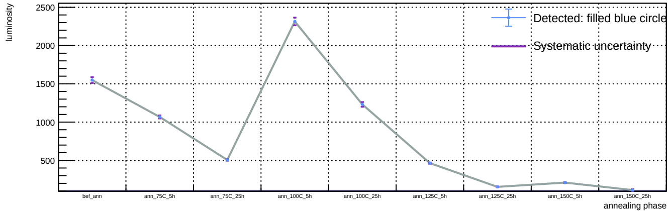
Sensor B1, T = 20 C, representative v = 55.9 V (max available) - Spot 53: luminosity vs phase
