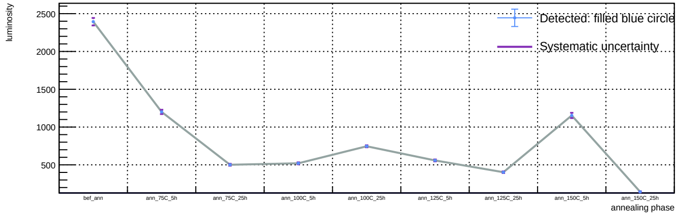
Sensor B1, T = 20 C, representative v = 55.9 V (max available) - Spot 60: luminosity vs phase
