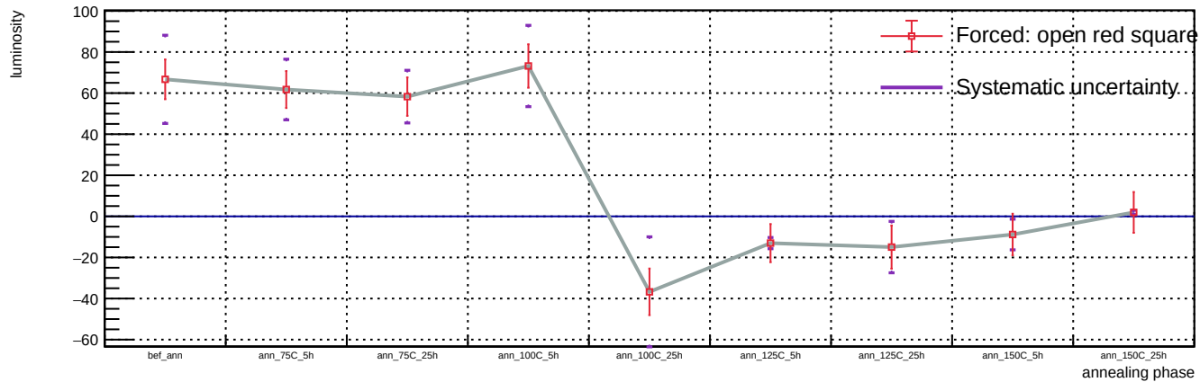
Sensor B1, T = 20 C, representative v = 55.9 V (max available) - Spot 73: luminosity vs phase
