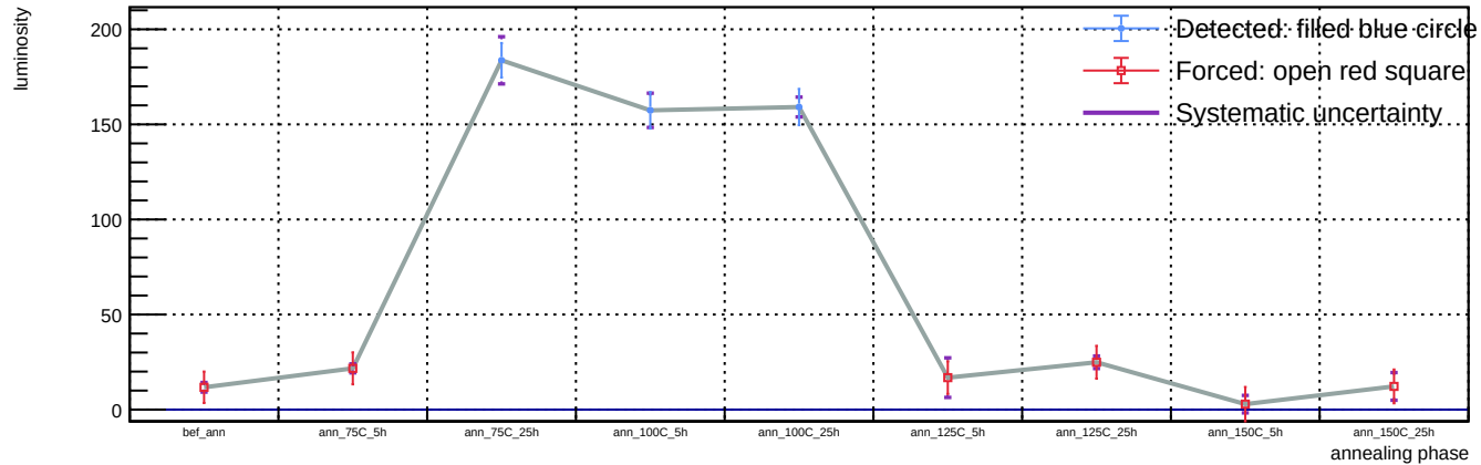
Sensor B1, T = 20 C, representative v = 55.9 V (max available) - Spot 76: luminosity vs phase
