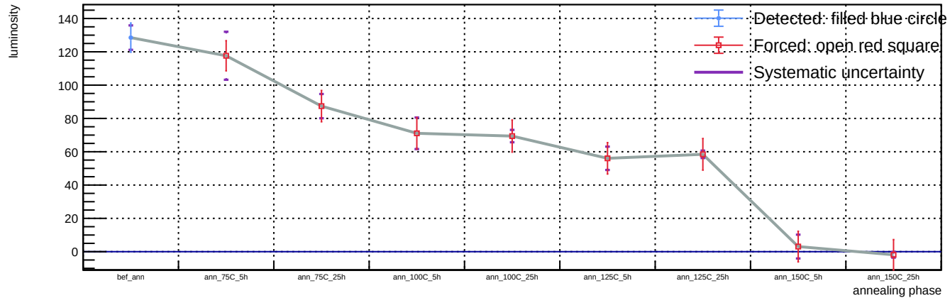
Sensor B1, T = 20 C, representative v = 55.9 V (max available) - Spot 8: luminosity vs phase
