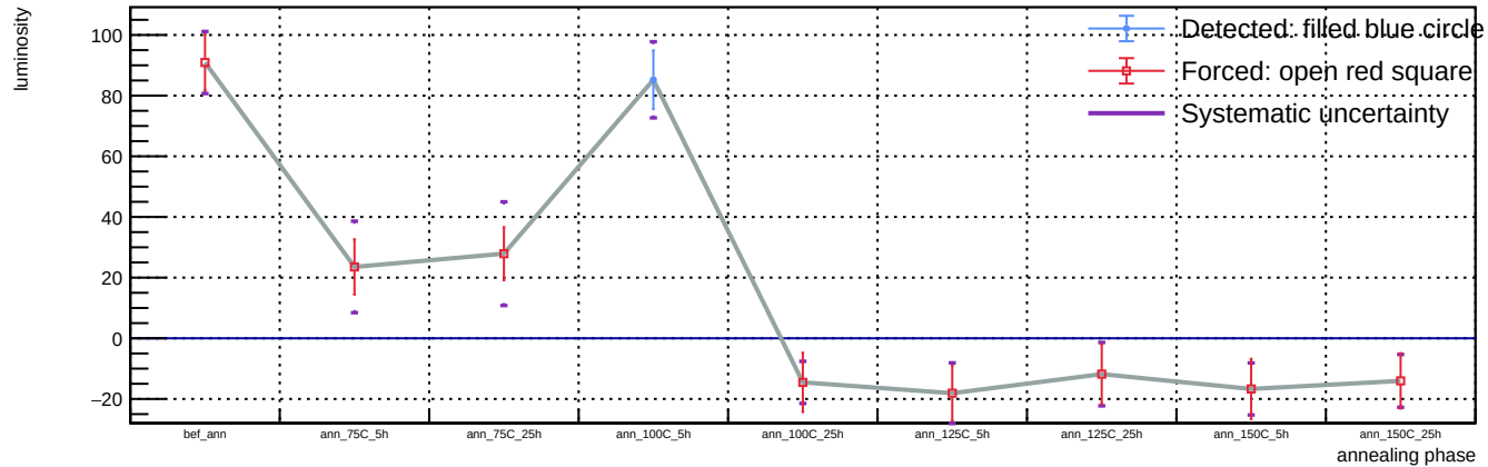
Sensor B1, T = 20 C, representative v = 55.9 V (max available) - Spot 81: luminosity vs phase
