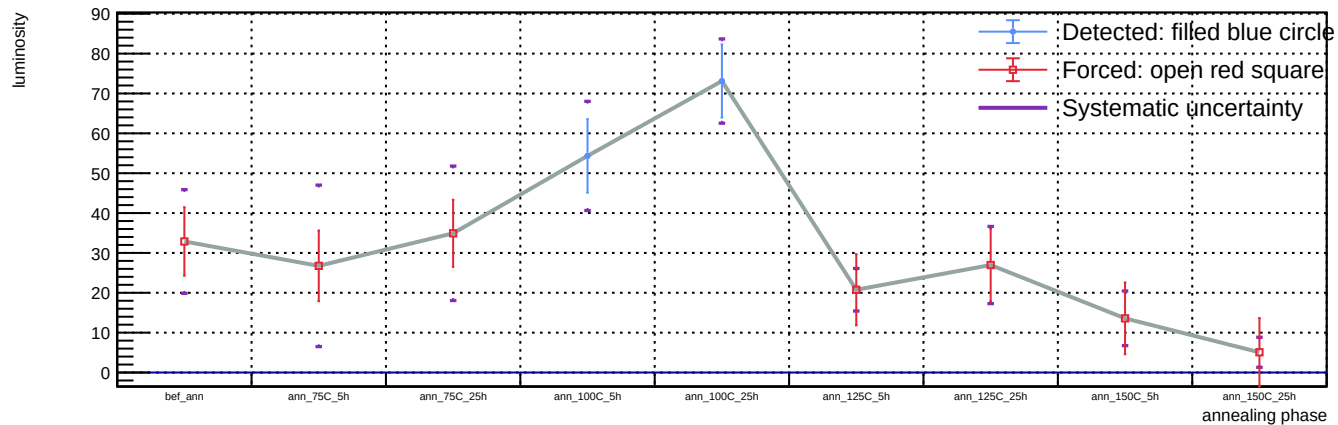
Sensor B1, T = 20 C, representative v = 55.9 V (max available) - Spot 82: luminosity vs phase
