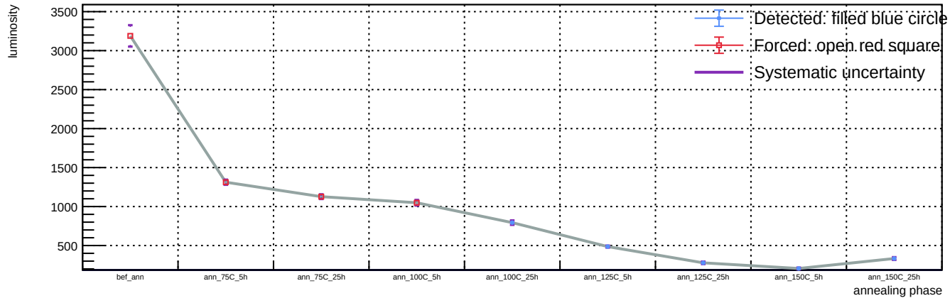
Sensor B1, T = 20 C, representative v = 55.9 V (max available) - Spot 85: luminosity vs phase
