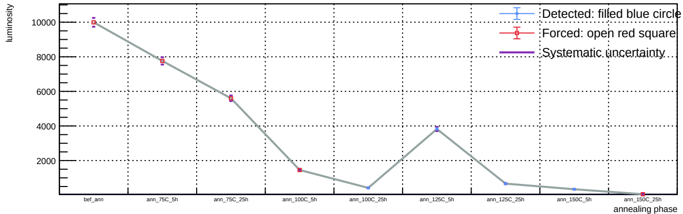
Sensor B1, T = 20 C, representative v = 55.9 V (max available) - Spot 89: luminosity vs phase
