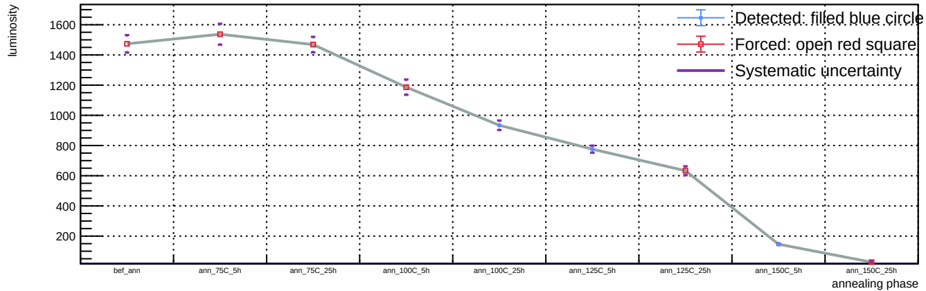
Sensor B1, T = 20 C, representative v = 55.9 V (max available) - Spot 90: luminosity vs phase
